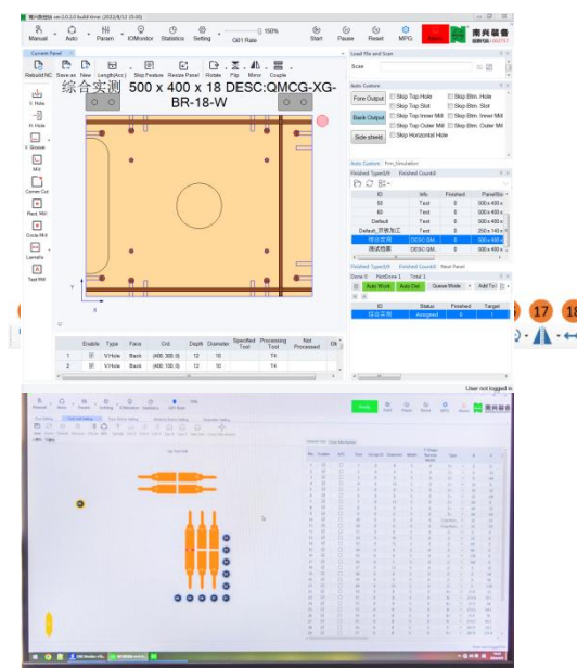
9.6 Drill Machine PC CAM - Auto Mode - Simulation
