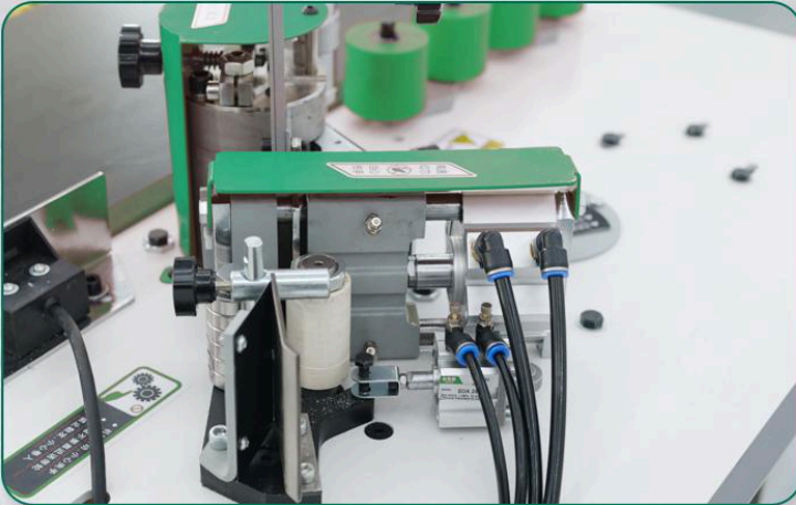
Brand new cutter assembly Compact structure, good cutting flatness effect
